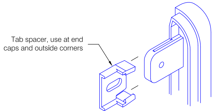
Spacer Detail
